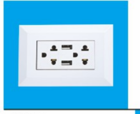
ZN 127 USB 5A 2.1V 15A 125V/250V
